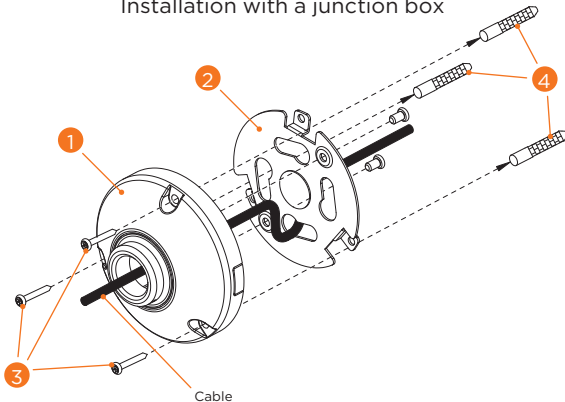
Installation with a junction box
